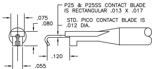
EXTENDED HOOK DETAIL
